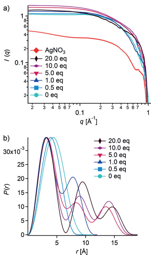
Figure 5. a) Log- q -log- I(q) X-ray scattering curves of 1 (50 mM) dissolved in acetonitrile with different concentrations of \text{AgNO}_3 , including a curve of \text{AgNO}_3 alone (50 mM), and b) the corresponding intensity-normalized PDDF spectra.
